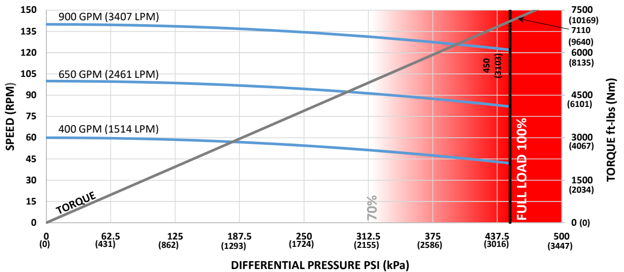
8 in (203mm) 7-8 Lobe 3.0 Stage
