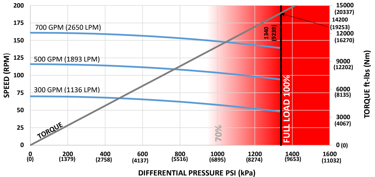
6.75 in (171mm) 7-8 Lobe 5.7 Stage HR
