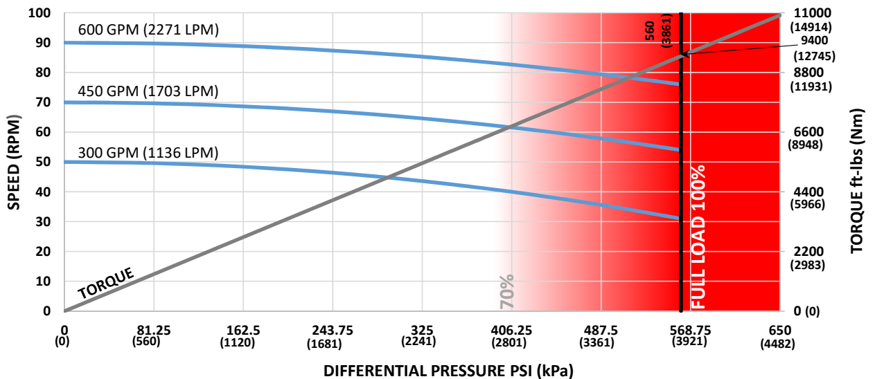
6.5 & 6.75 in (165 & 171mm) 7-8 Lobe 3.3 Stage HR
