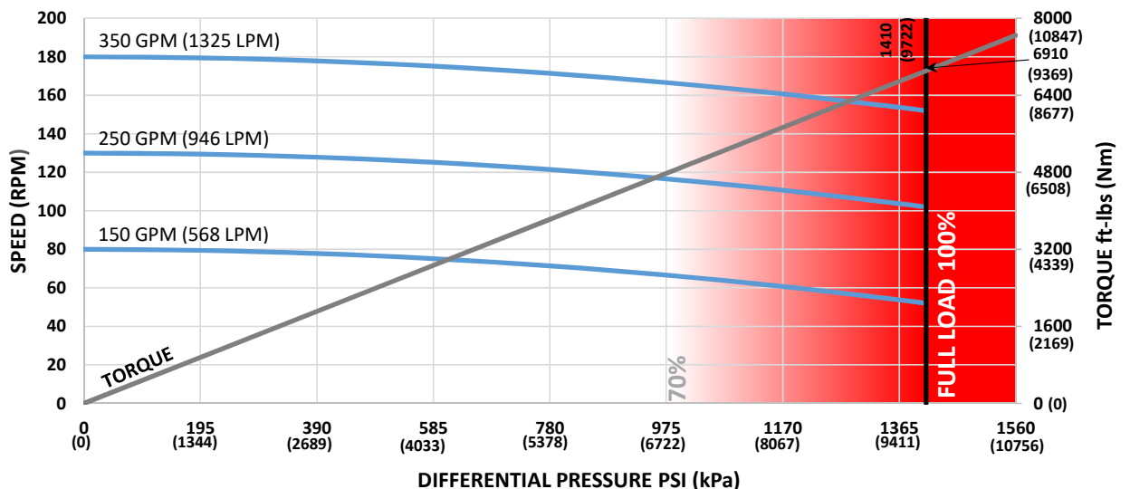
5 in (127mm) 8-9 Lobe 6.0 Stage HR
