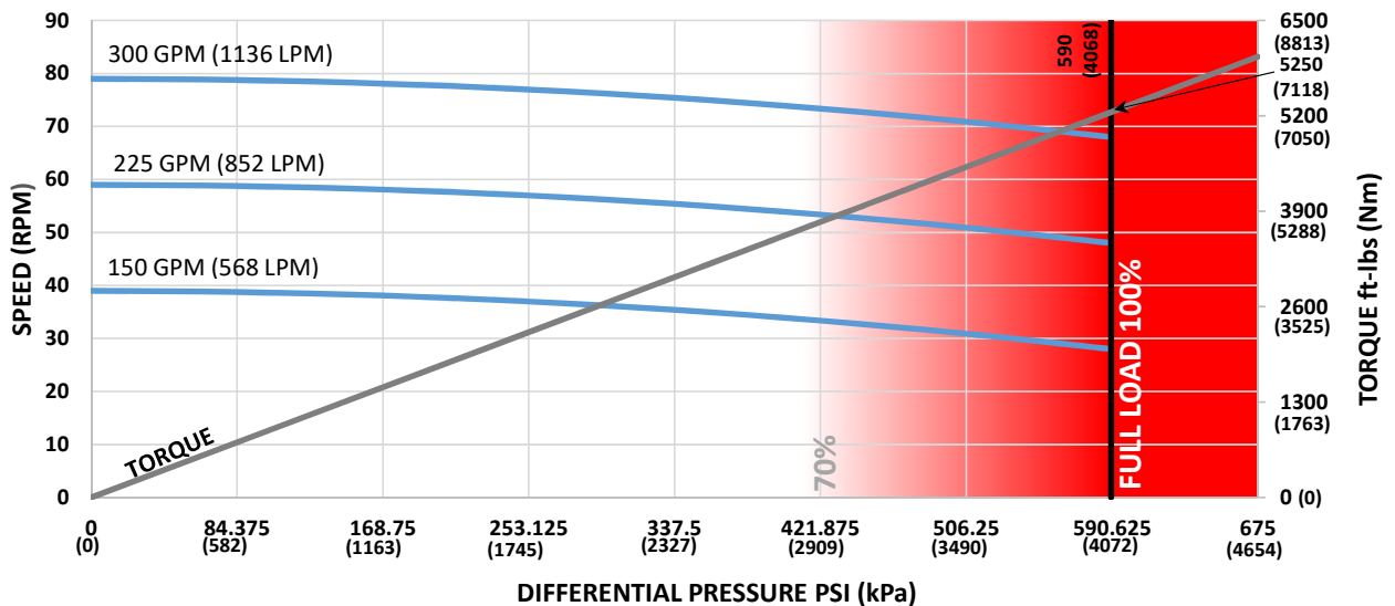
5 in (127mm) 7-8 Lobe 2.6 Stage HR
