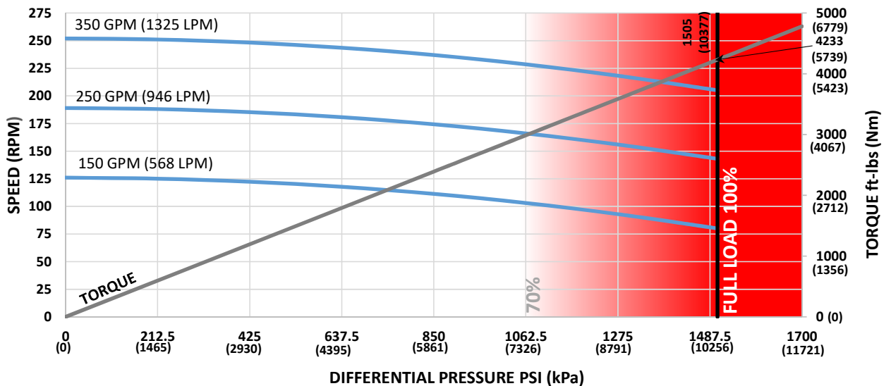
5 in (127mm) 6-7 Lobe 6.0 Stage HR
