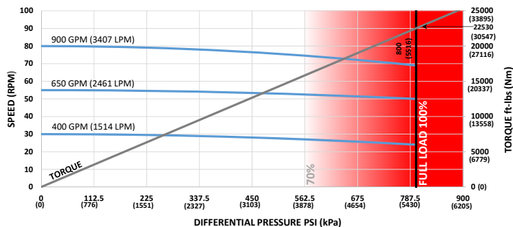
8 in (203mm) 7-8 Lobe 3.4 Stage HR
