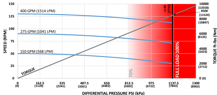
6.5 &amp; 6.75 in (165 &amp; 171mm) 7-8 Lobe 4.8 Stage HR
