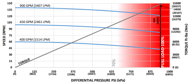
8 in (203mm) 7-8 Lobe 4.0 Stage HR
