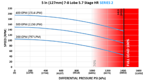
Speed Chart (See page 29)
