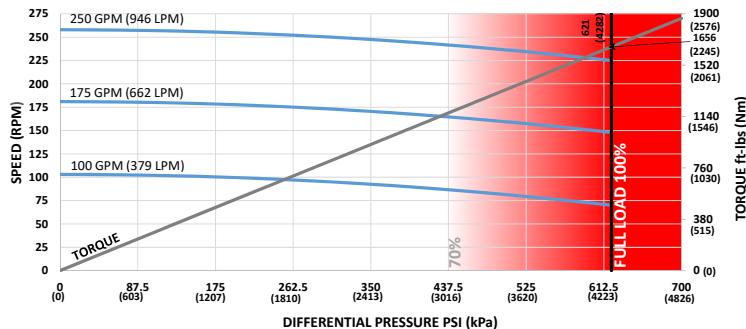
5 in (127mm) 5-6 Lobe 4.0 Stage HR
