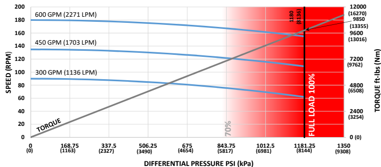
6.5 &amp; 6.75 in (165 &amp; 171mm) 6-7 Lobe 5.0 Stage HR
