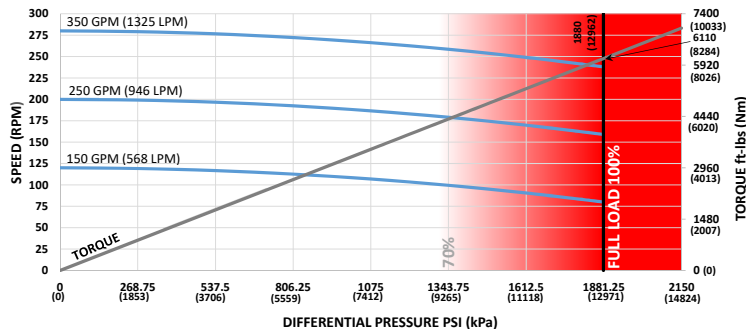
5 in (127mm) 6-7 Lobe 8.0 Stage HR
